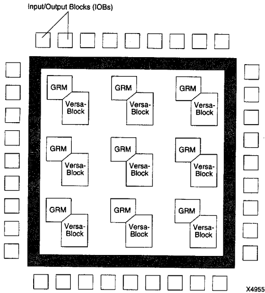
Figure 1: XC5200 Architectural Overview
