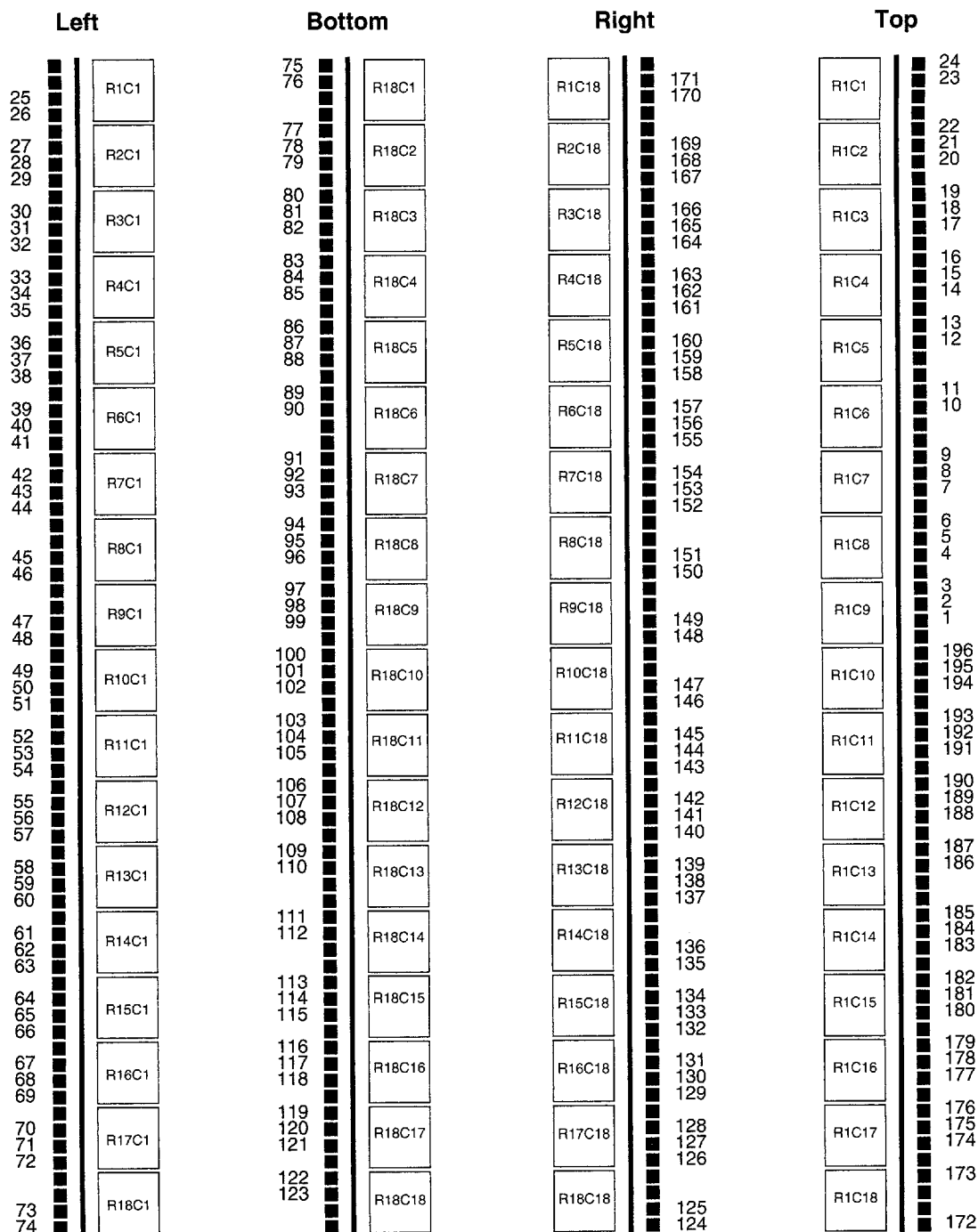
Figure 25: XC5210 CLB-to-Pad Relationship (Detail)
