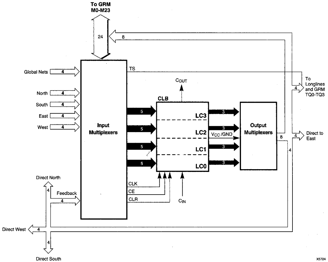
Figure 10: VersaBlock Details
