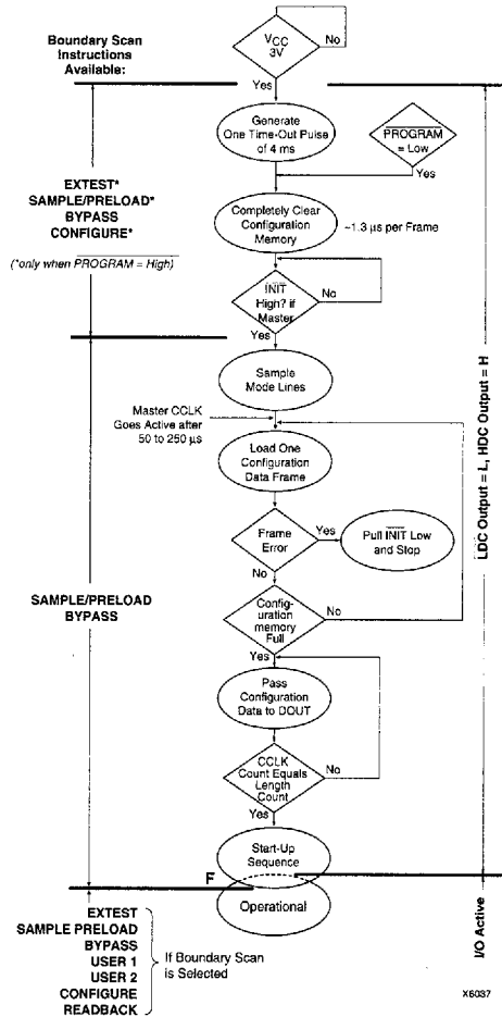
Figure 17: Configuration Sequence
